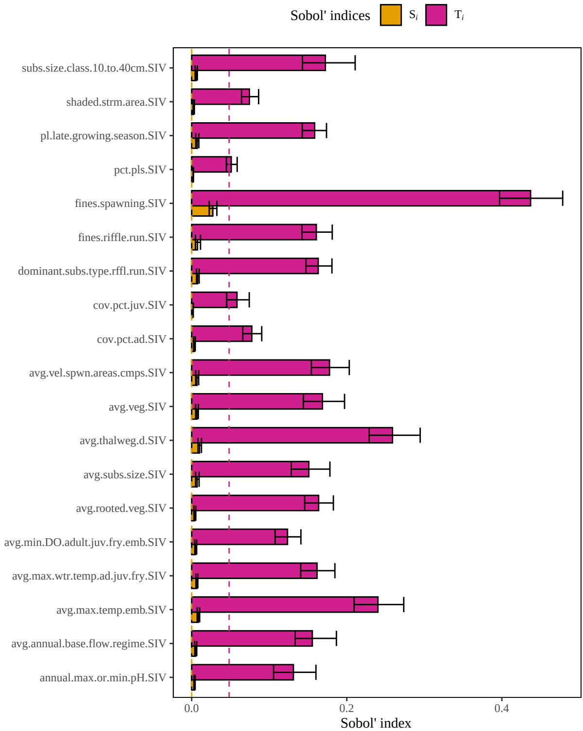
Figure 7. Results of a sensitivity analysis for the cutthroatRivLahontanLtoe15CMt5m model based on a multiplicative mean structure. Dashed lines represent baseline numerical approximation error for S_i and T_i ( i.e. , dummy variables).
